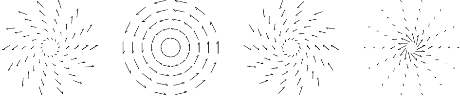
Figure 1. (xOz) -velocity field. From left to right: (a_1, a_2, a_3, a_4) = (0, 0.75, 0, 1) , (0, 1, 0, 1) , (0, 2, 0, 1) and (1, 1, 0, 1) .
