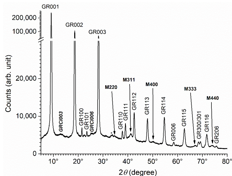
Figure 7. XRD pattern of the precipitate obtained with acetate after 1 week of ageing at RT. GR = \text{GR}(\text{SO}_4^{2-}) , GRCI = \text{GR}(\text{Cl}^-) , M = magnetite, with the corresponding Miller index. * = unidentified peaks.
